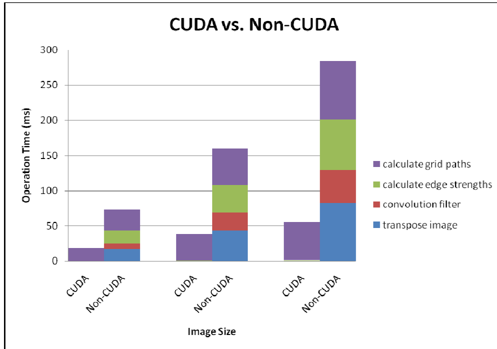
Figure 4.6: Comparisons of runtime of each task in CUDA and before optimizations. Note the CUDA executions of the edge strengths, convolution filter, and transpose operations are too fast to be visible on this timescale.
