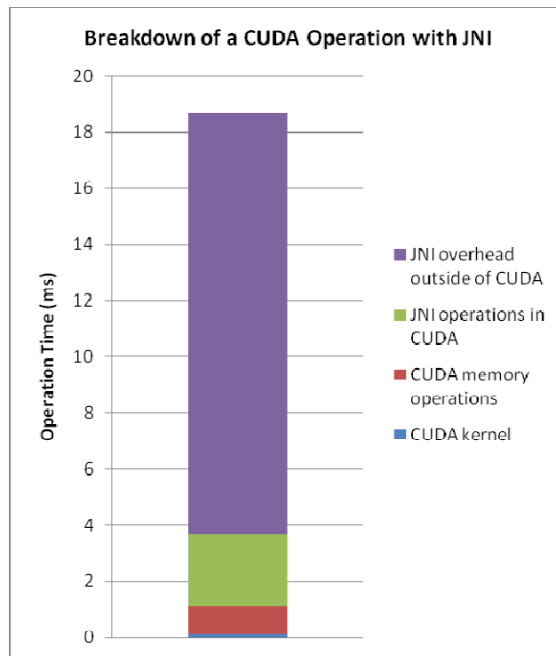
Figure 5.1: The benchmarks of each subsection of the transpose operation on a sample 400x304 image. The CUDA kernel, the sliver at the bottom, is the data presented in this paper. The CUDA memory operations are necessary, though unoptimized. The JNI operations and overhead will be removed entirely in future work.
