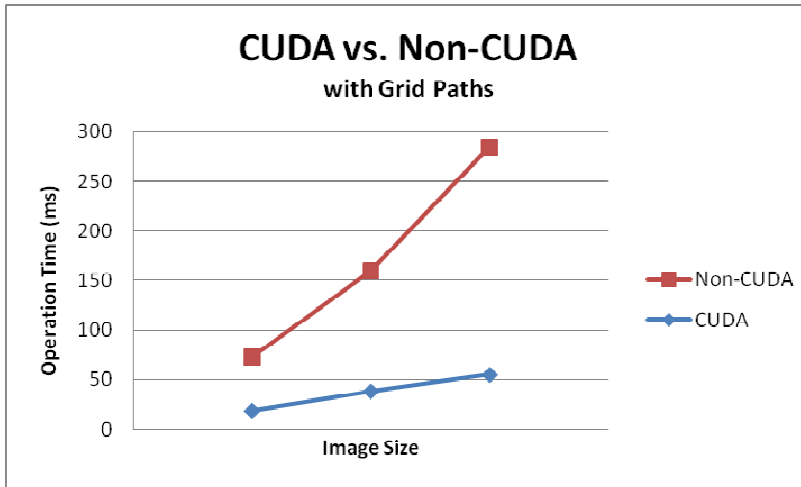
Figure 4.4: Summation of time required to execute the re-implemented segments of PathFinder by CUDA and by the original Java code. Includes the grid paths calculation.
