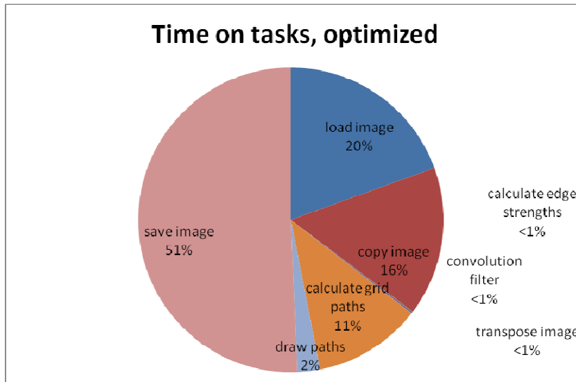
Figure 4.7: Each task performed by PathFinder, as percentage of runtime post-CUDA enhancements.
