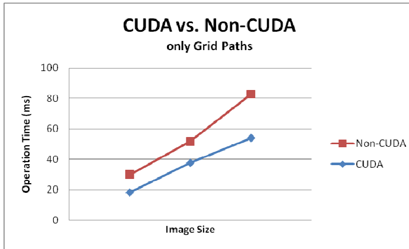
Figure 4.3: Time required to execute the grid paths calculation by CUDA and by the original Java code.
