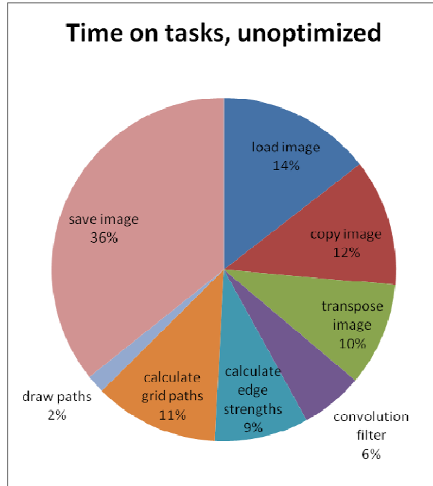
Figure 4.1: Each task performed by PathFinder algorithm, as percentage of runtime.
