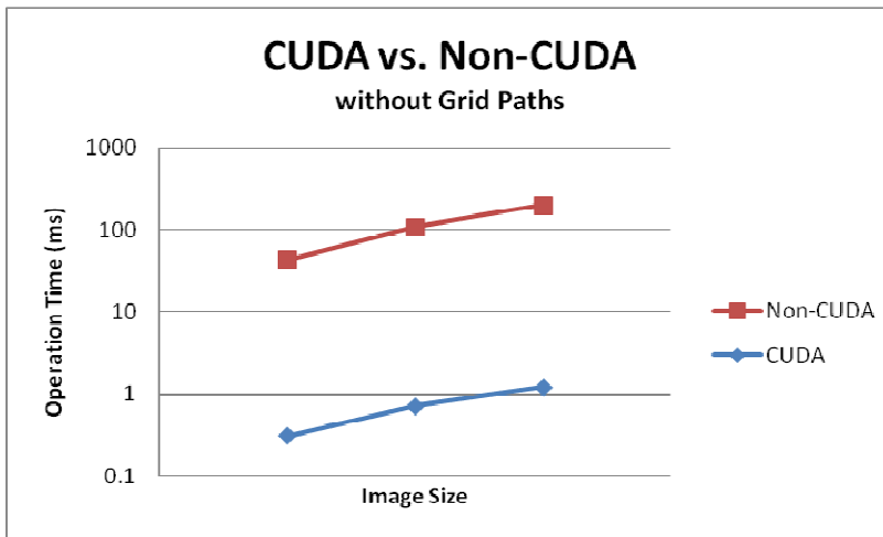
Figure 4.5: Summation of time required to execute the re-implemented segments of PathFinder by CUDA and by the original Java code. Does not include the grid paths calculation.
